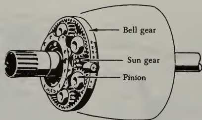
Spur-planetary
